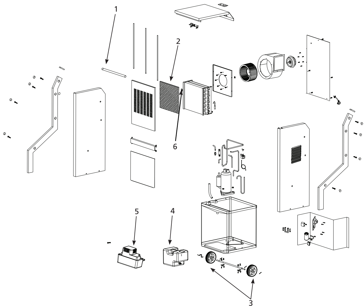
Figure 5 – Repair Parts Illustration for Dehumidifiers
